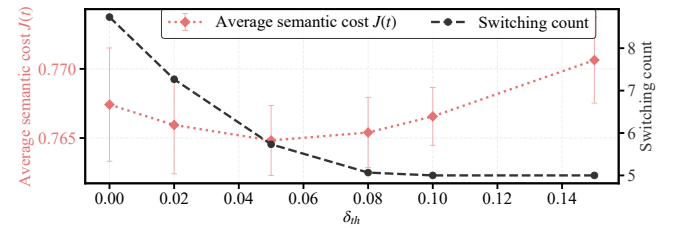
Figure 10: Sensitivity to Hysteresis Threshold.
