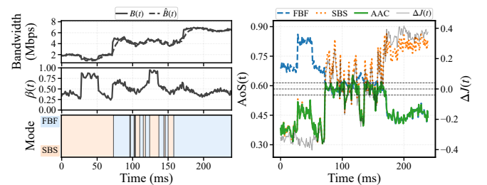
Figure 7: Real time control under temporal variations.
