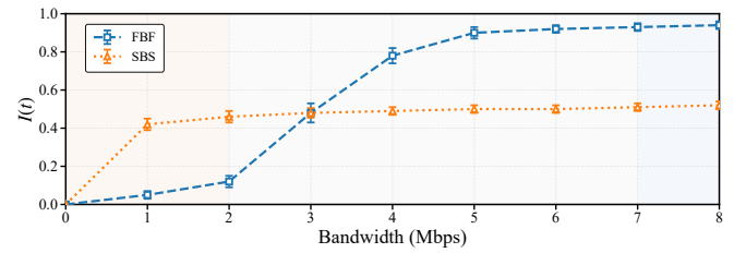
Figure 6: Semantic complementarity of FBF and SBS.
