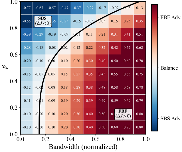
Figure 4: Decision space.
