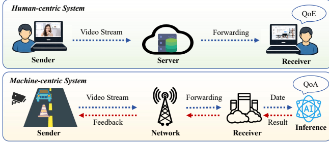
Figure 1: Differences between Human-centric and Machine-centric Streaming Transmission Systems.
